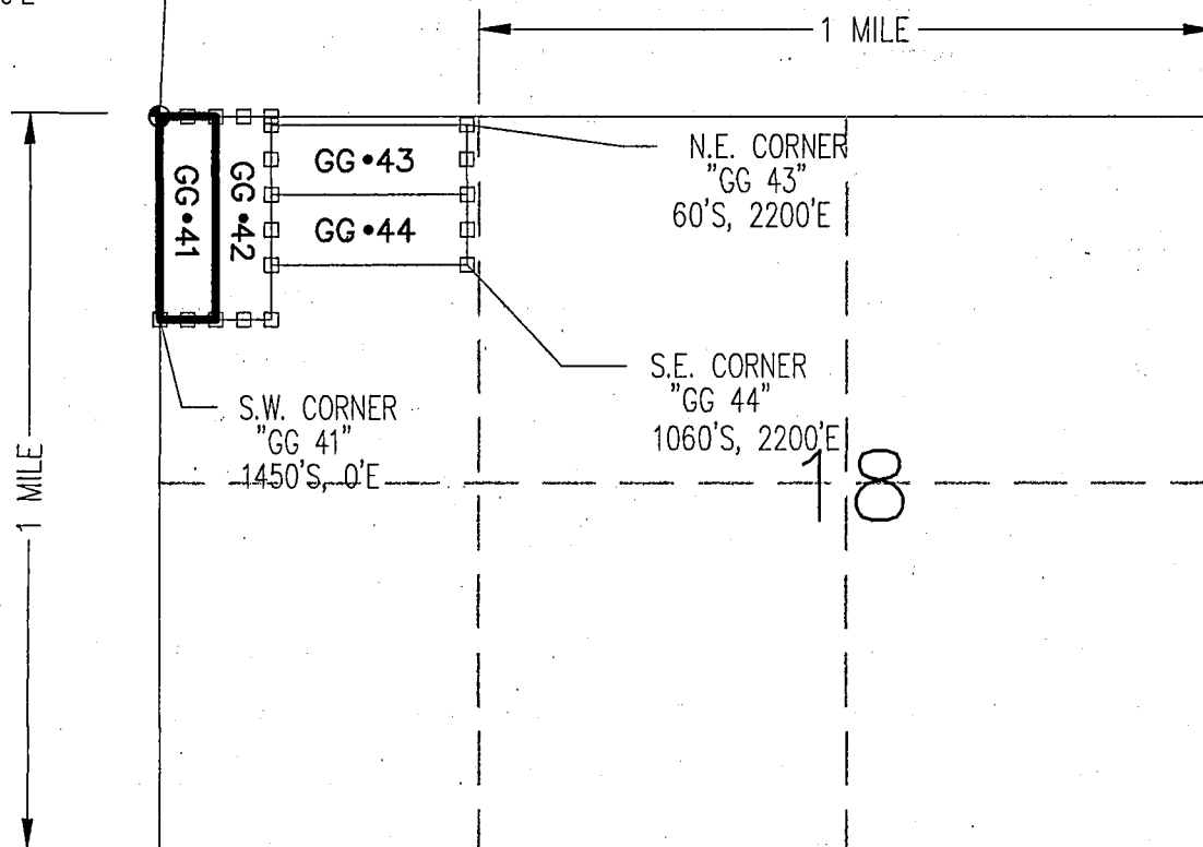
"GG 41" CLAIM DETAIL (NOT TO SCALE)
