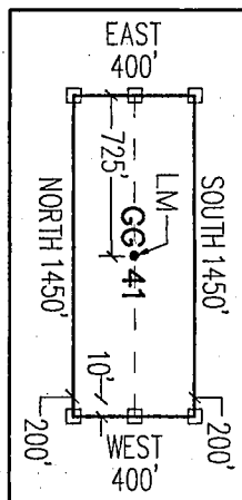
"GG 41" CLAIM DETAIL (NOT TO SCALE)
